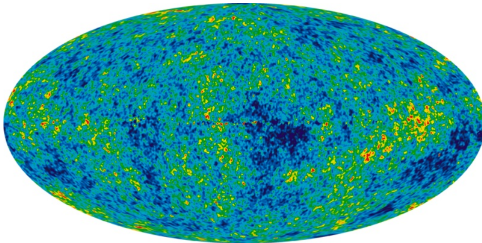
The Universe as it appeared just 380,000 Years after the Big Bang
